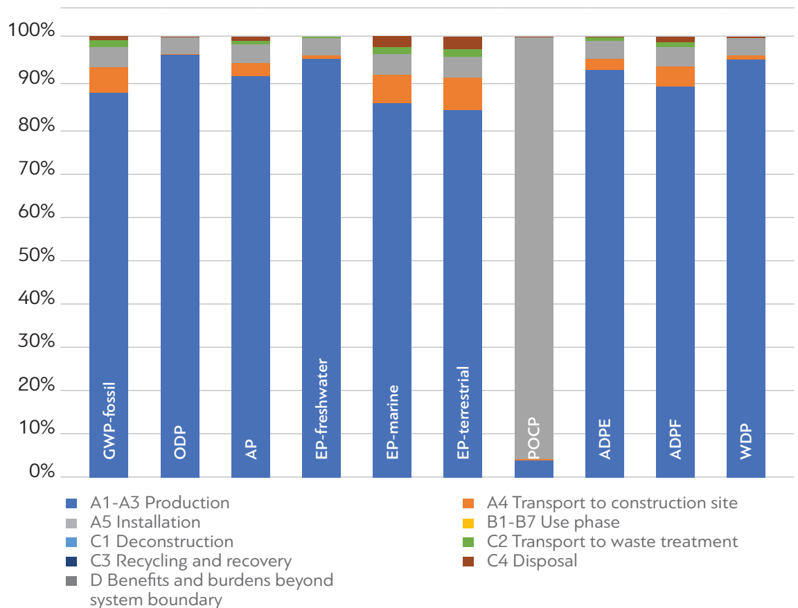
Figure 1: Environmental impacts of ClimaTop® Classic finishing render (impacts A1-C4 = 100 %) The largest part of environmental impacts is caused during production (modules A1-A3). It is only for the photochemical oxidation potential, where the VOC emissions during curing contribute significantly to module A5.
